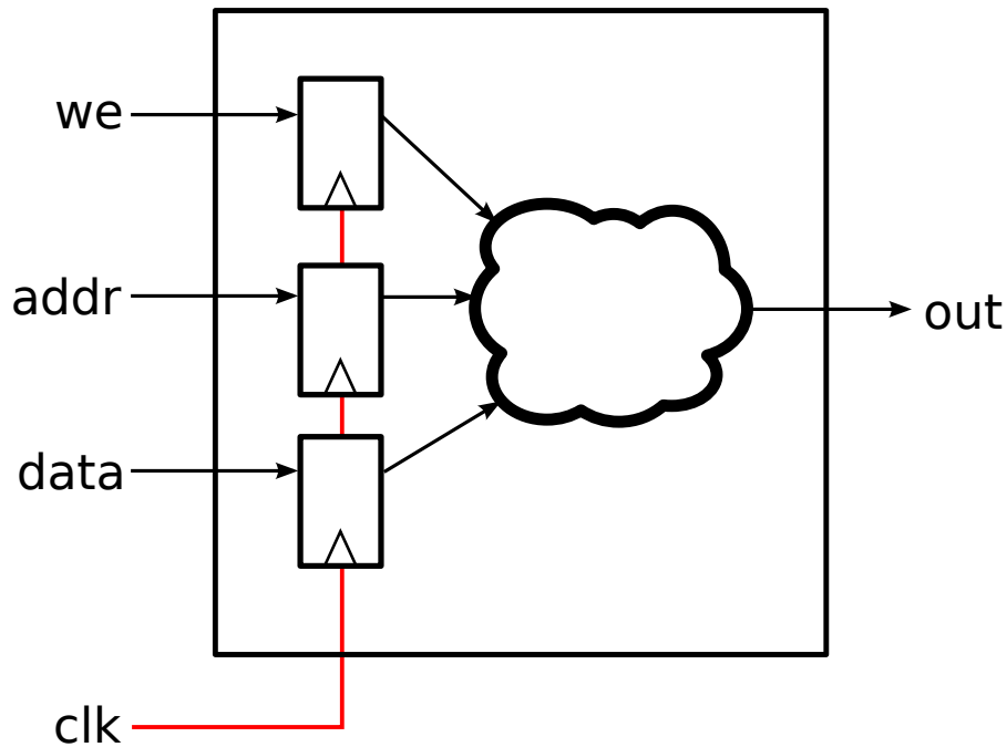
Fig. 6.12: Mixed sequential/combinational single port ram
