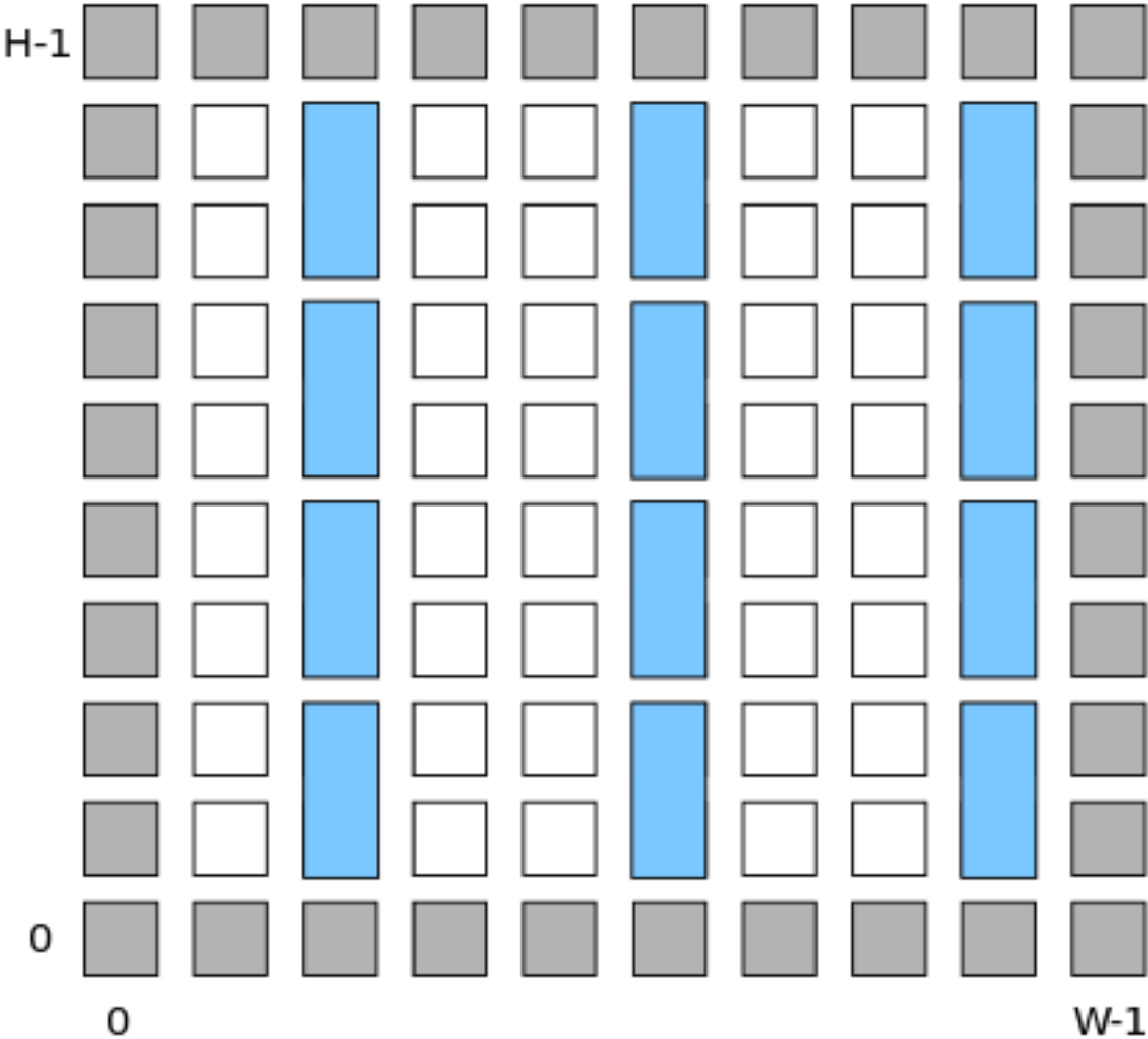
Fig. 2.6: <col> RAM and <perimeter> io example
