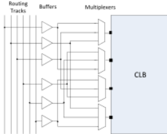
Fig. 1.5: Connection Box
